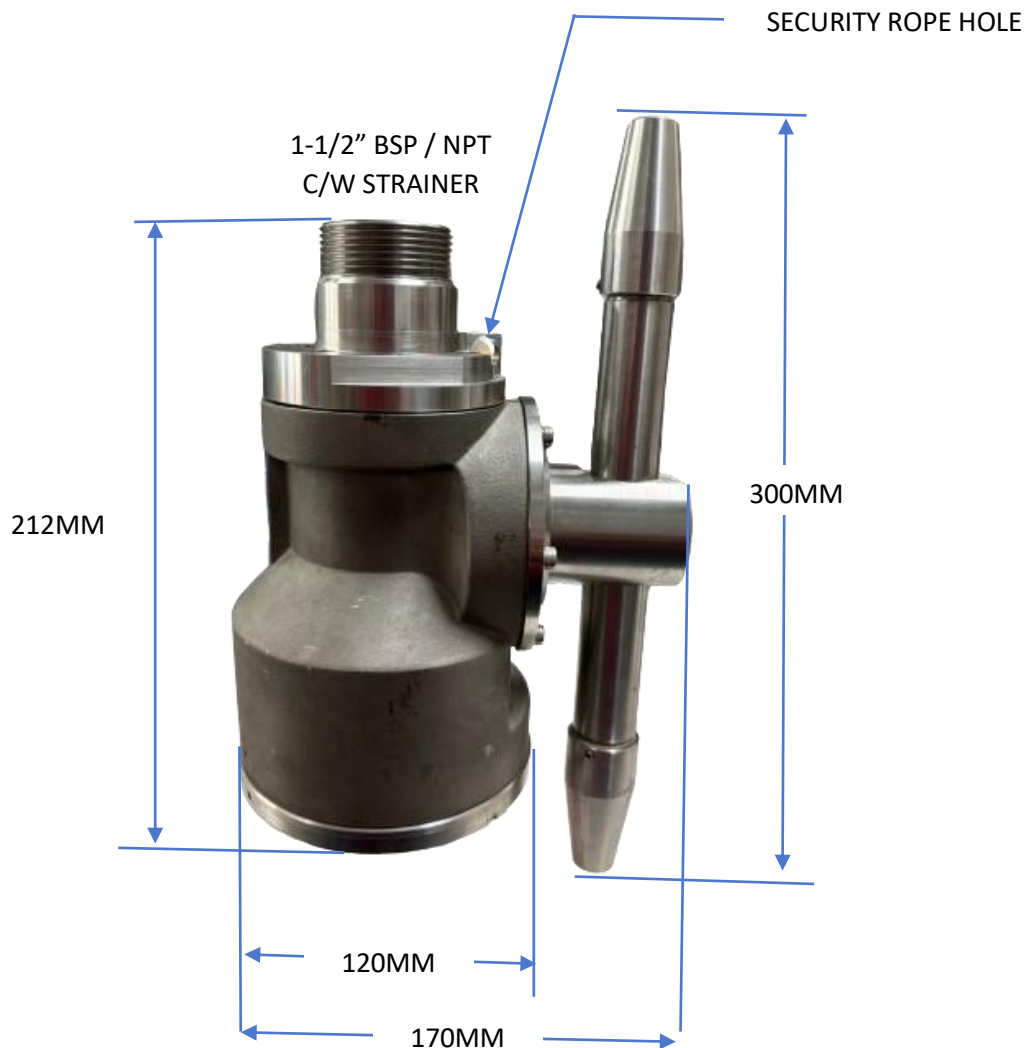
XB12P DIMENSIONS
